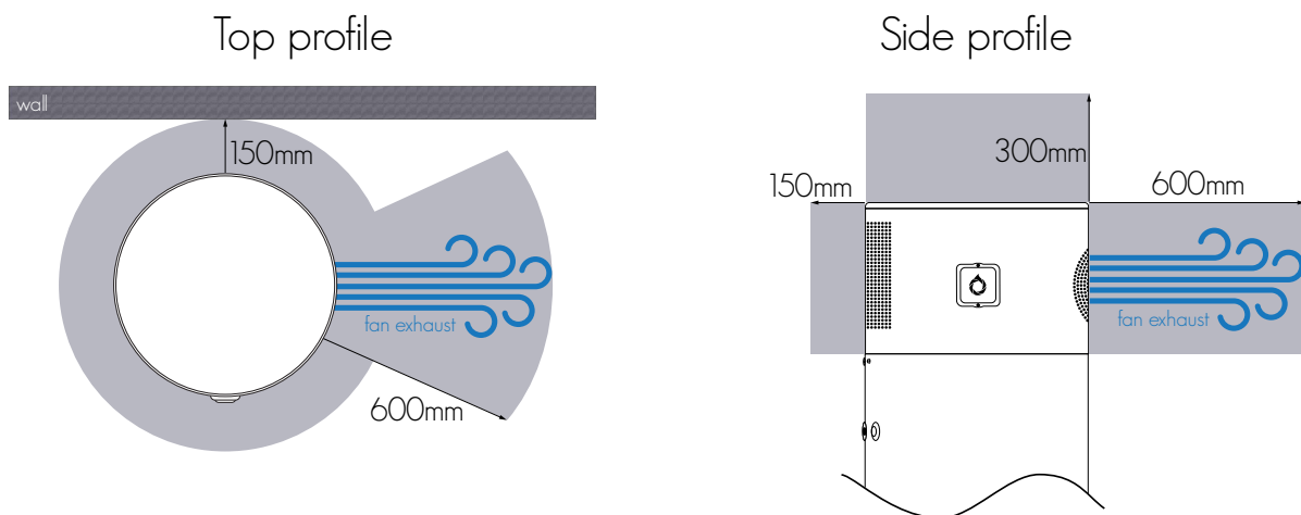
Figure 2: Front profile of DYNAMIC/X8 installation requirements.
